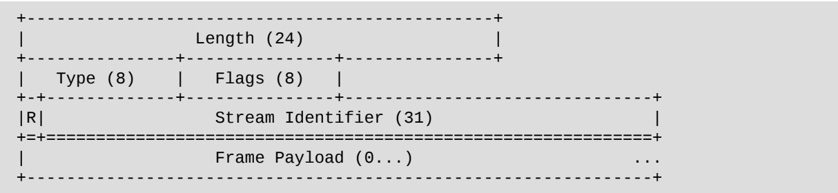
Figure 1: Frame Layout
